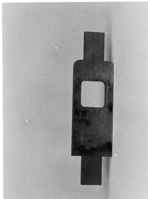
FIG. 1 Shearing Tool
